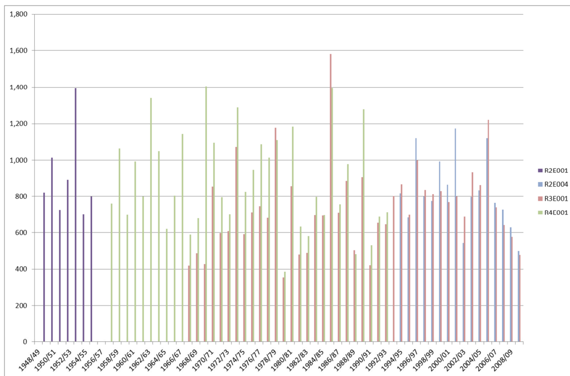
Figure 5-15 Annual rainfall [mm/a] for different weather stations in RU2; a) within R2 secondary catchments, b) around East London (includes R3 and R4 catchments)
