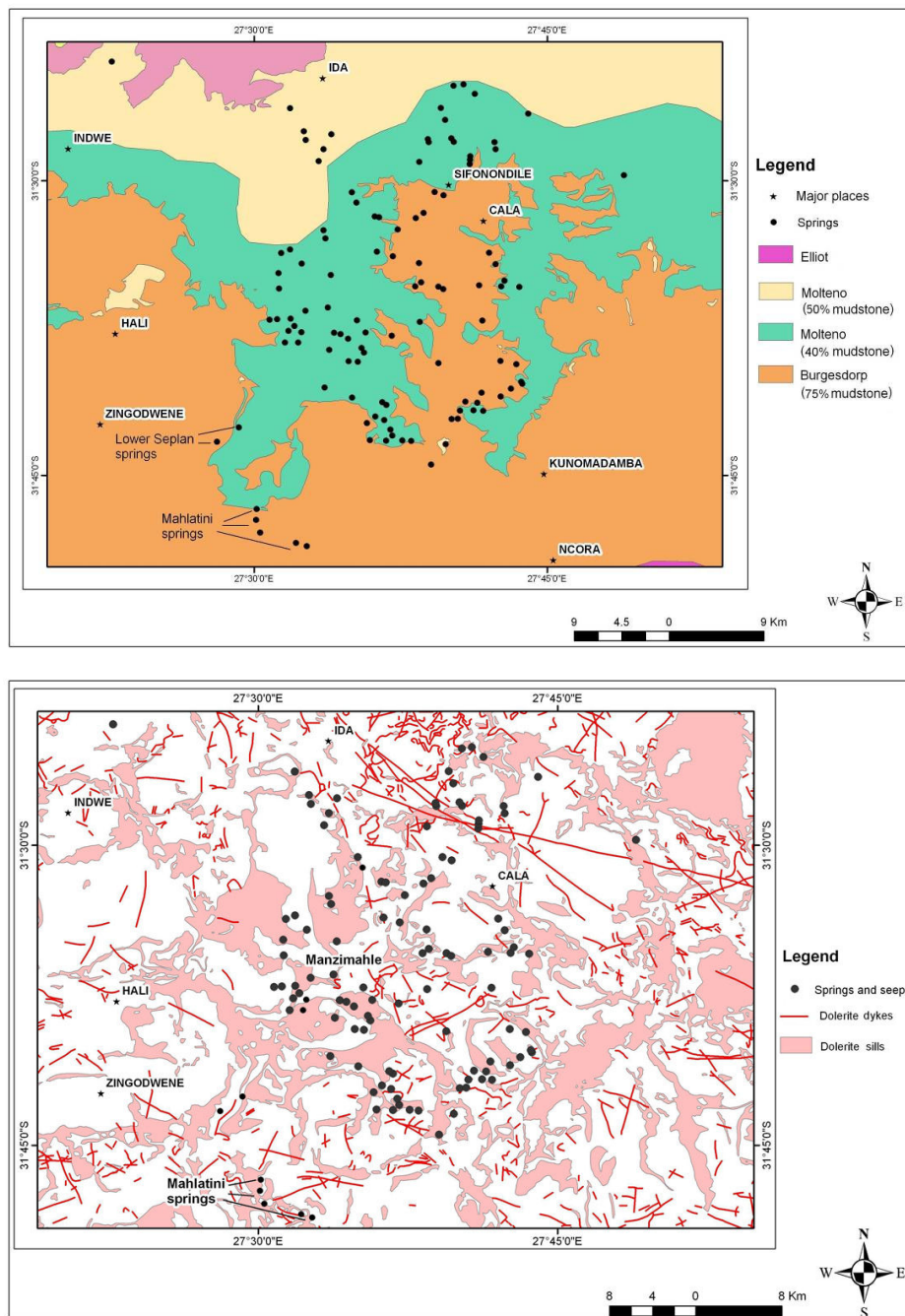
Figure 5-69 Distribution of springs of the Manzimahle area (Resource Unit 13; a) with respect to the Burgersdorp – Molteno contact; b) with respect to dolerite sills (from Chevallier et al, 2010)
