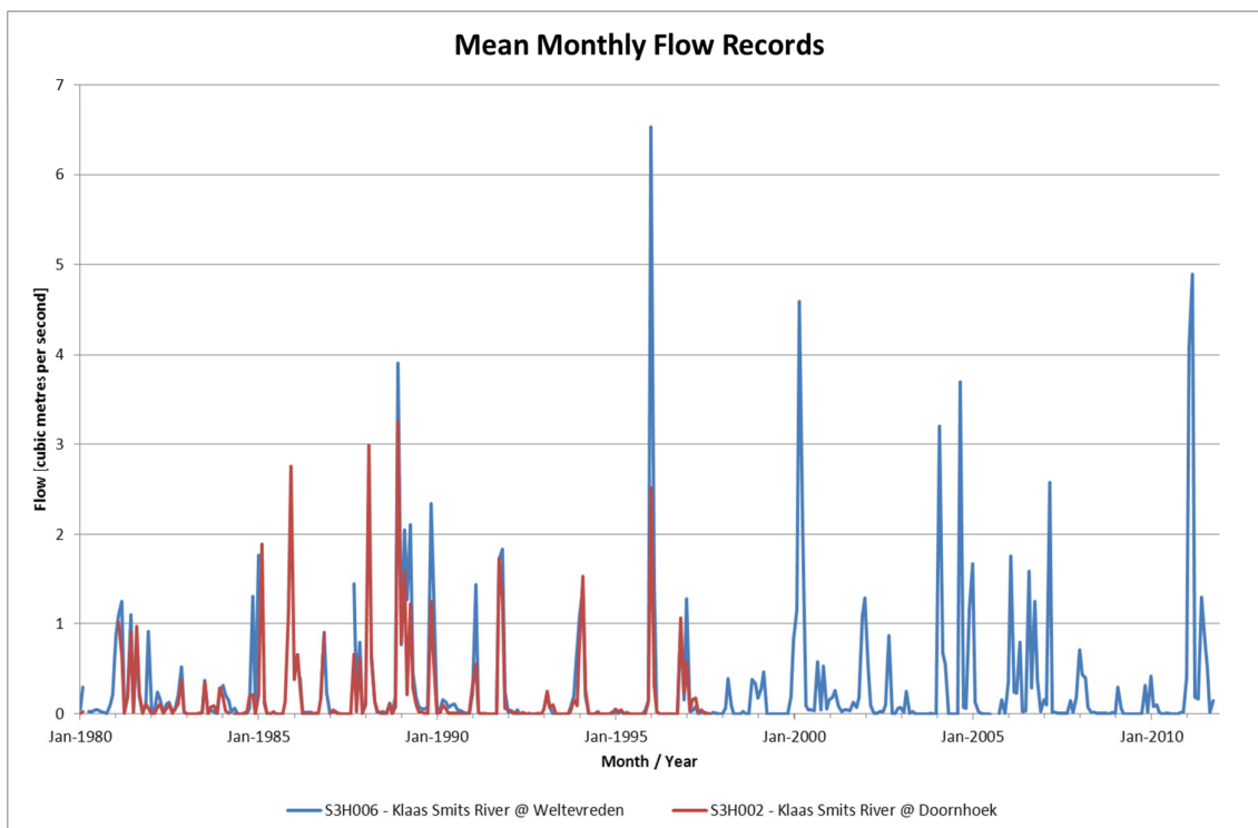
Figure 5-74 River hydrographs in RU14 to 22; a) Black Kei River, b) Klaas Smits River
