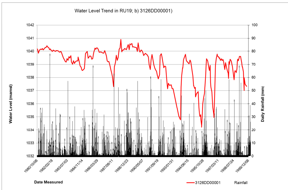
Figure 5-84 Water level trends in selected boreholes from RU19; a) 3126DC00001, 3126DC00002 & 3126DC00003; b) 3126DD00001
