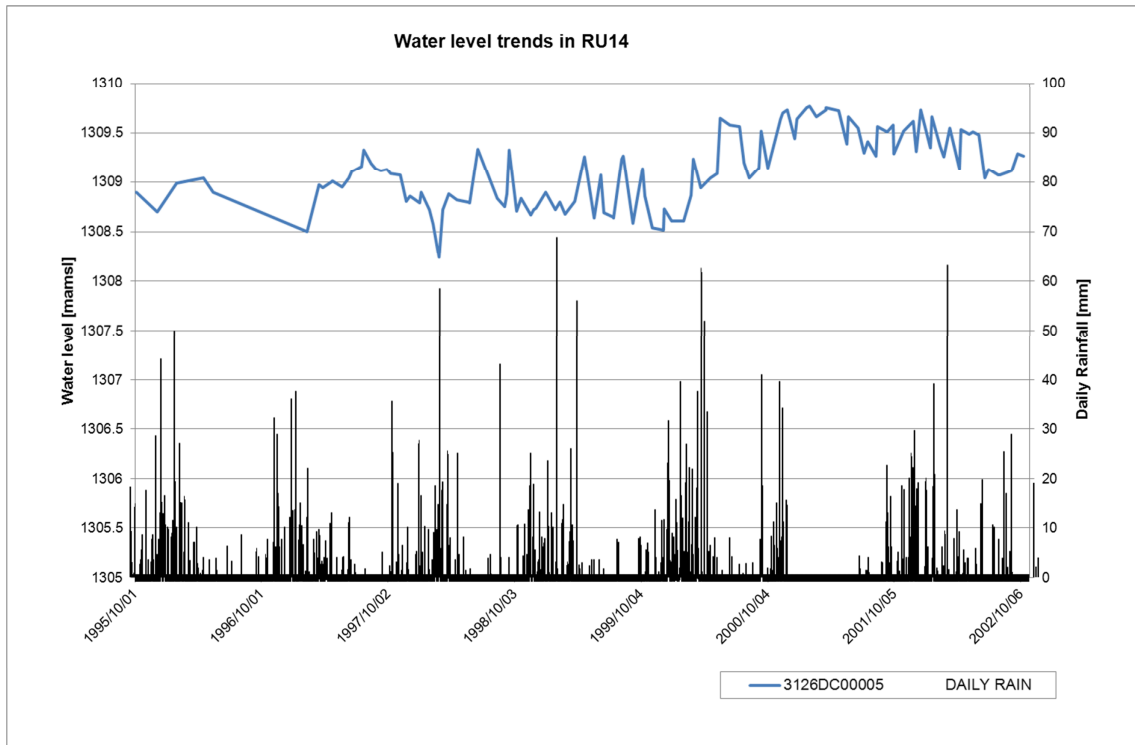
Figure 5-81 Water level trends in selected borehole from RU14 (3126DC00005)
