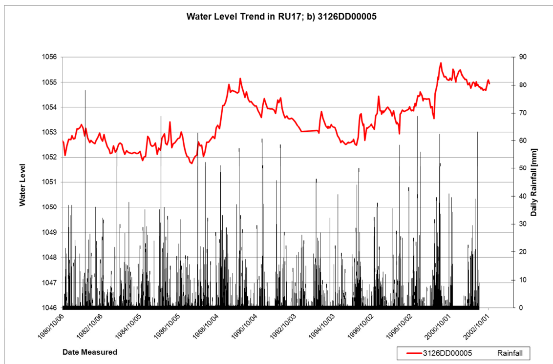
Figure 5-83 Water level trends in selected boreholes from RU17; a) 3126DD00003, b) 3126DD00005
