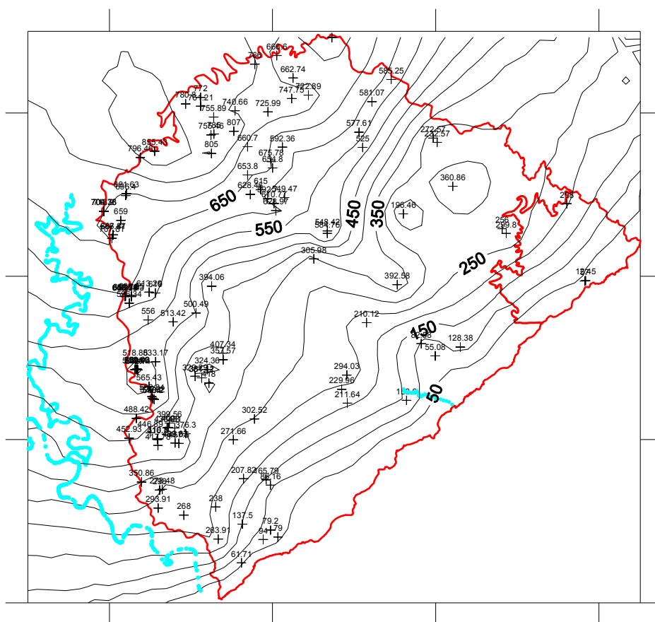
Figure 5-36 Piezometric map for RU4
