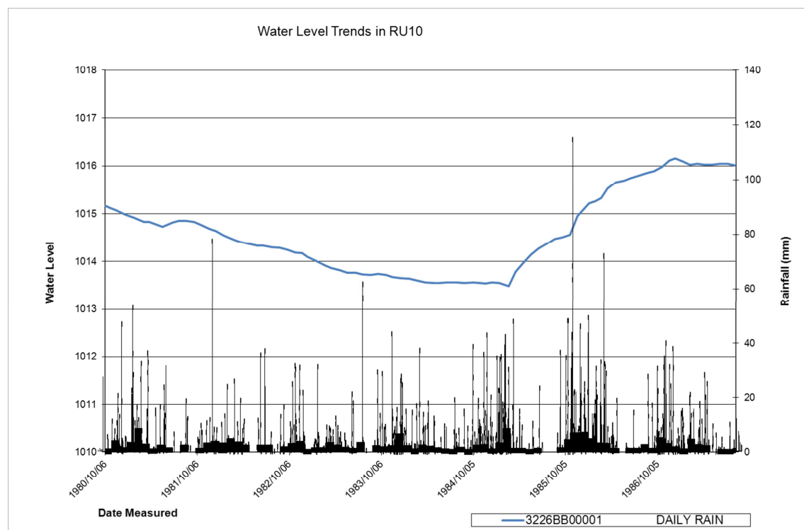
Figure 5-56 Water level trends in selected borehole from RU10
