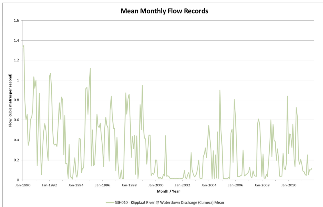
Figure 5-53 River hydrographs in RU10; a) Black Kei River along profile, b) Klipplaat River downstream of Waterdown Dam
