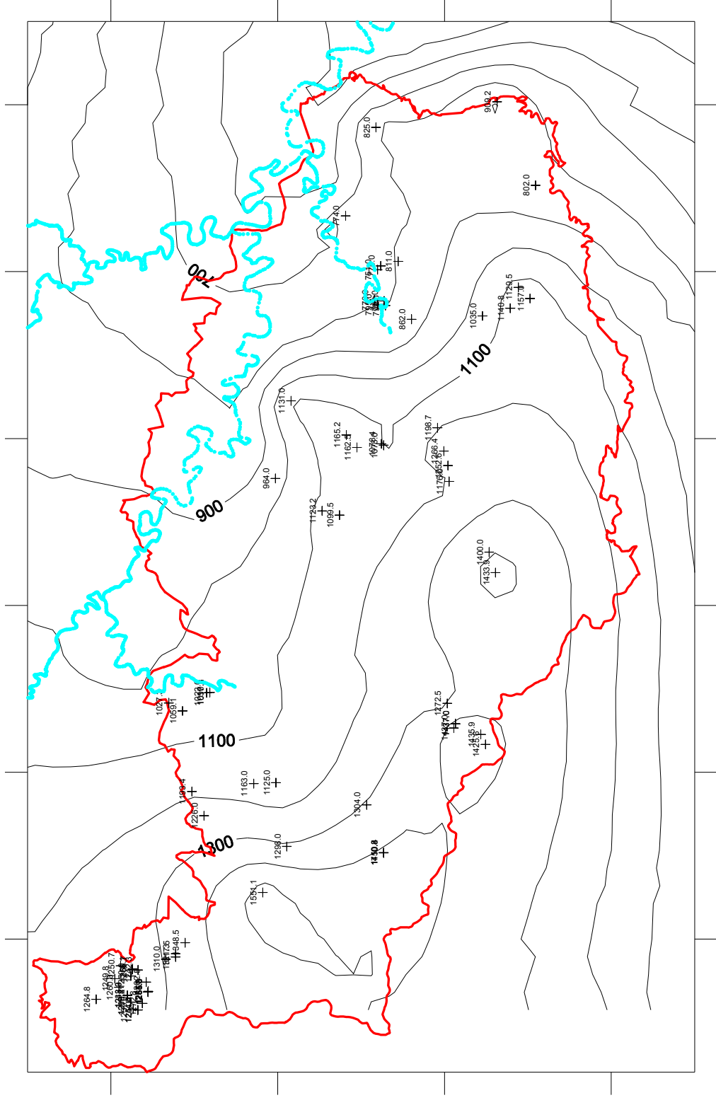
Figure 5-55 Piezometric map for RU10
